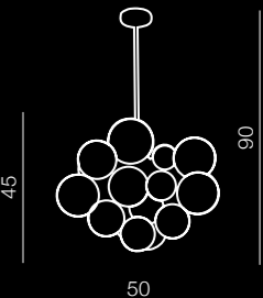
Noble AZ0110 G4 10x 20W 12V metal/glass chrome/white
