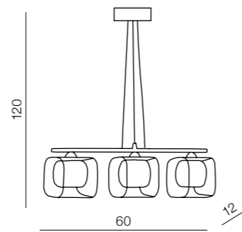
Happy 3 AZ0484 G9 3x 40W metal/chrome/glass clear/glass white
