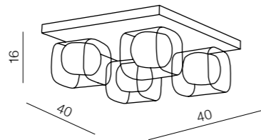
Happy 4 top AZ0485 G9 4x 40W metal/chrome/glass clear/glass white
